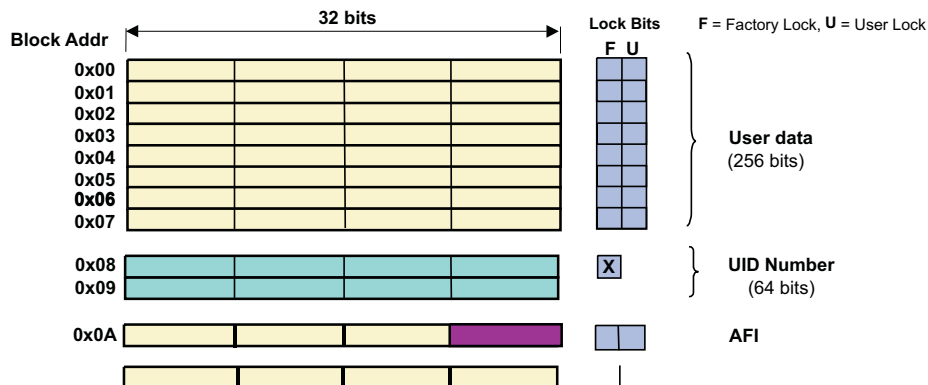
Figure 1-2. Memory Organization of the Tag-it HF-I Standard Transponder IC
